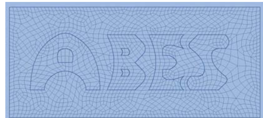
Various options for mesh refinements, curved edges
